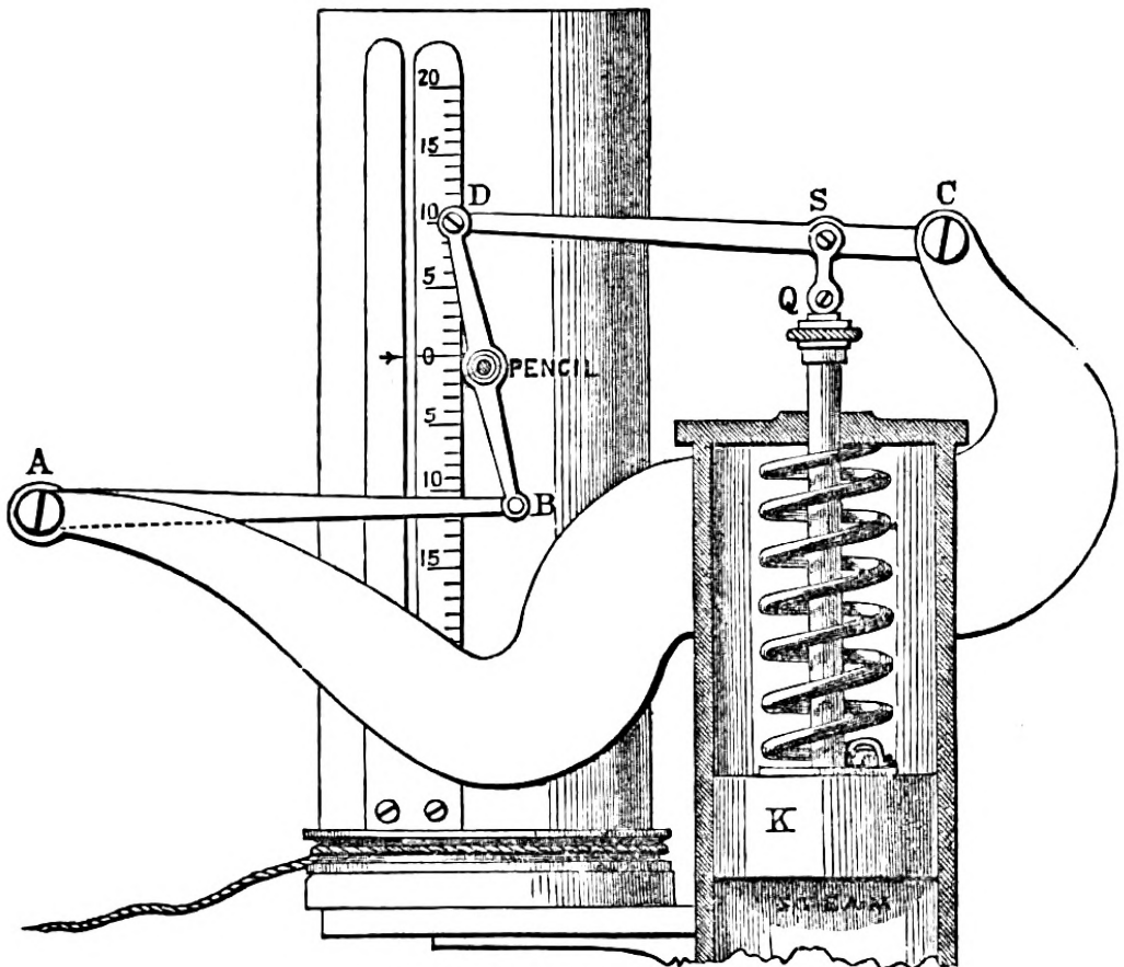
Richards's Indicator.
