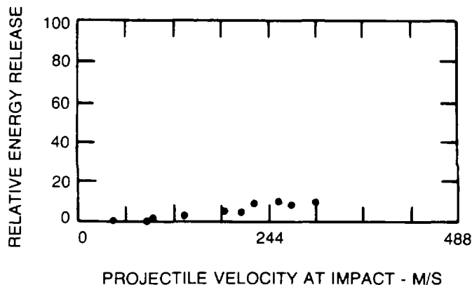
Figure 8-52. Susan test results for TATB.
