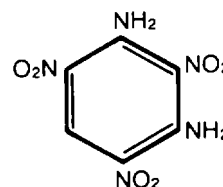
Figure 8-43. Structural formula for DATB.
