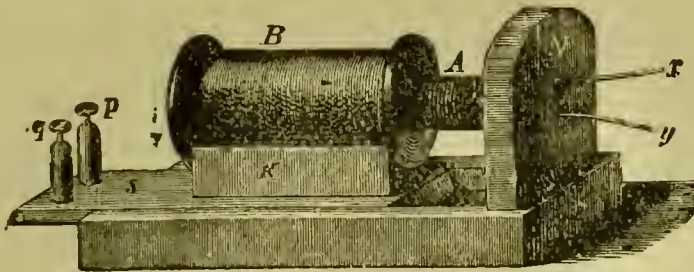
FIG. 10. INDUCTION COIL.
