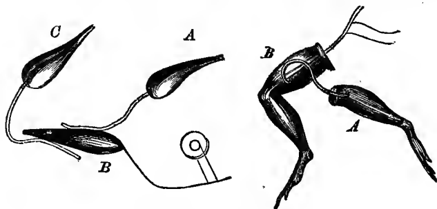
FIG. 57 & 58. SECONDARY PULSATION.
