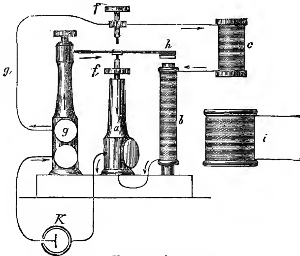
FIG. 74. HELMHOLTZ'S APPARATUS.
