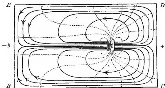
FIG. 44. CURRENT-CURVES AND TENSION-CURVES.
